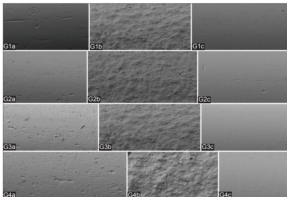
Figure 5: Representative scanning electron microscope images of wire surfaces in different studied groups. (G1a: DW + NiTi wire; G1b: DW + coated wire; G1c: DW + SS wire; G2a: NaF + NiTi wire; G2b: NaF + coated wire; G2c: NaF + SS wire; G3a: CHX + NiTi wire; G3b: CHX + coated wire; G3c: CHX + SS wire; G4a: ZM + NiTi wire; G4b: ZM + coated wire; G4c: ZM + SS wire).
