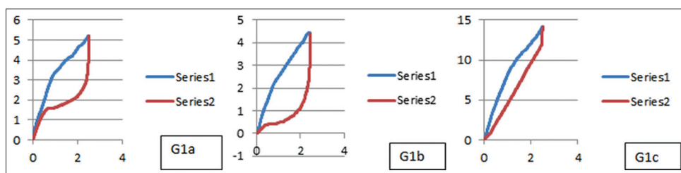
Figure 4: Load-deflection curve for three subgroups of control group (G1). (G1a: DW + NiTi wire; G1b: DW + coated wire; G1c: DW + SS wire).
