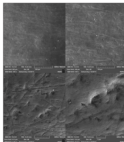
Figure 3: The scanning electron microscopy micrographs taken from the Group 2 (laser-activated gel + 980 nm laser).
